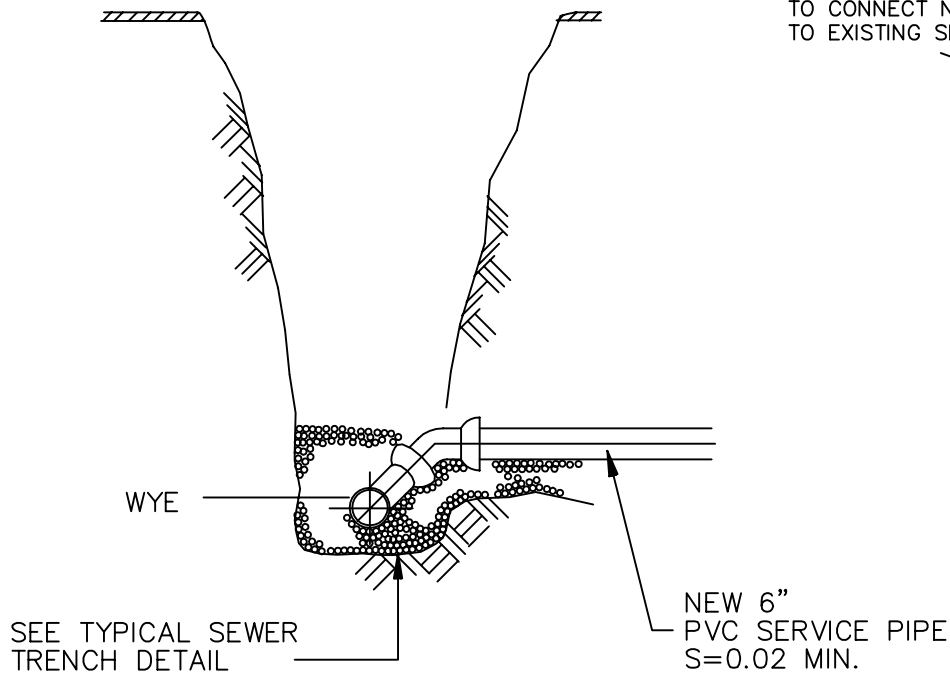
TYPICAL NEW WYE TO EXISTING SEWER CONNECTION DETAIL N.T.S.
