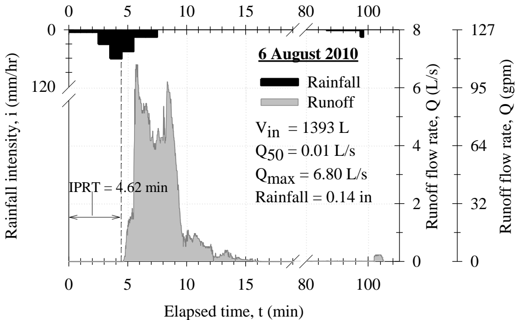
Figure B7: Hydrograph and hyetograph for 6 August 2010 event
